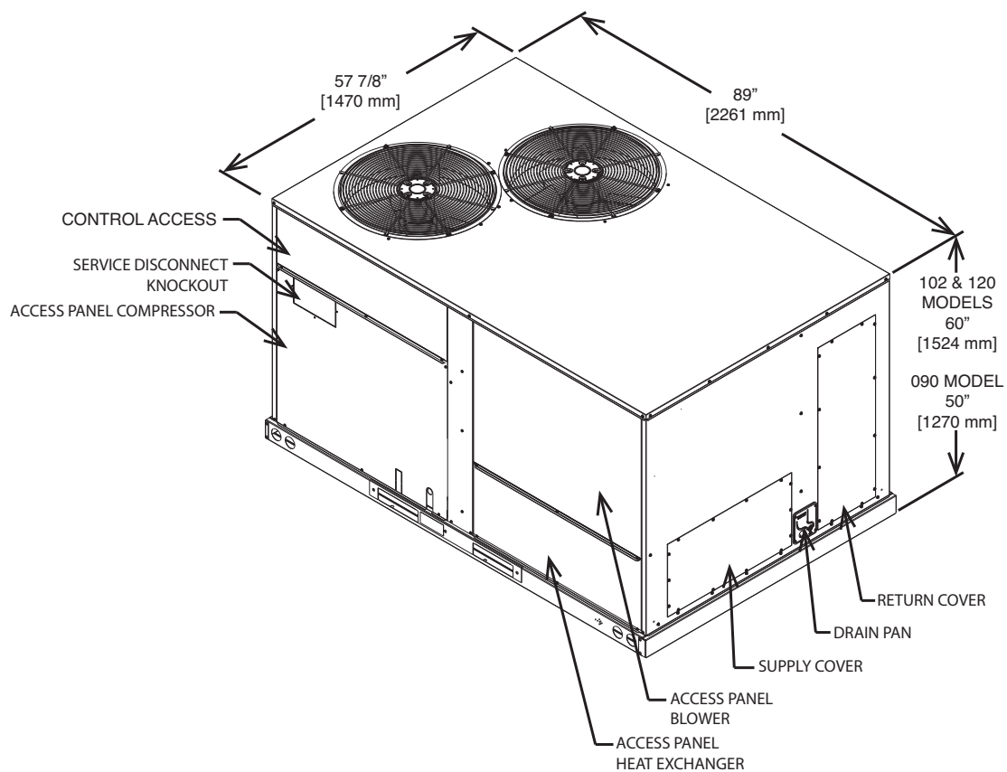
Illustration ST-A1273-26_B-00
